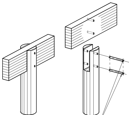
Broches LAMELLIX types L.BRL.1
